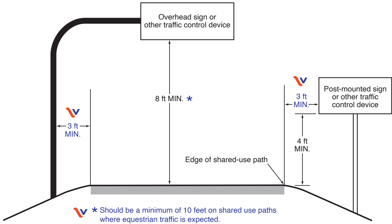
Figure 9A-1(VA). Sign Placement on Shared-Use Paths
