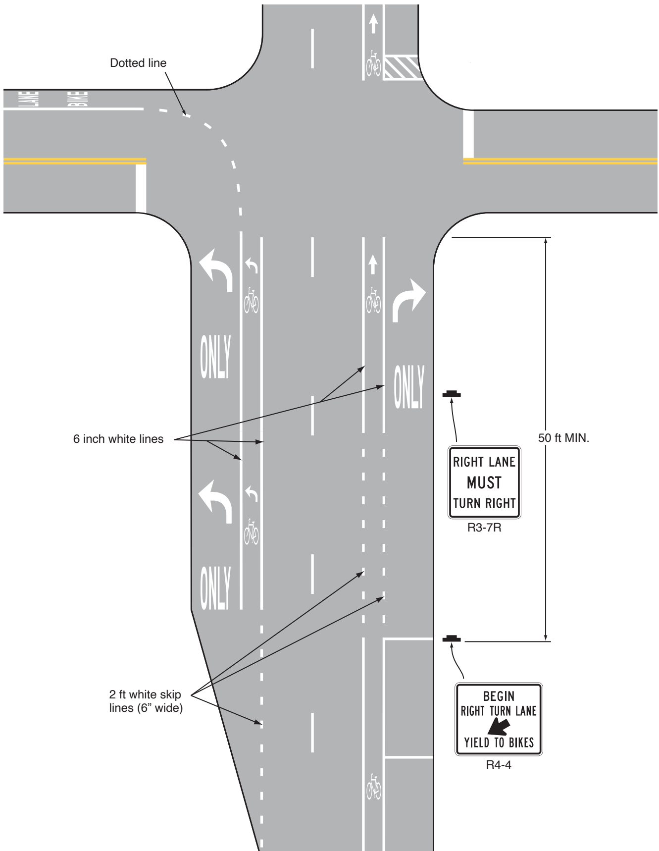
Figure 9E-3(VA). Examples of Bicycle Lane Markings on an Approach to an Intersection (Sheet 3 of 3)
