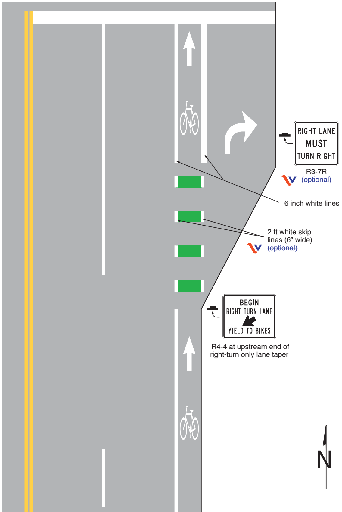
Figure 9E-3(VA). Examples of Bicycle Lane Markings on an Approach to an Intersection (Sheet 1 of 3)
