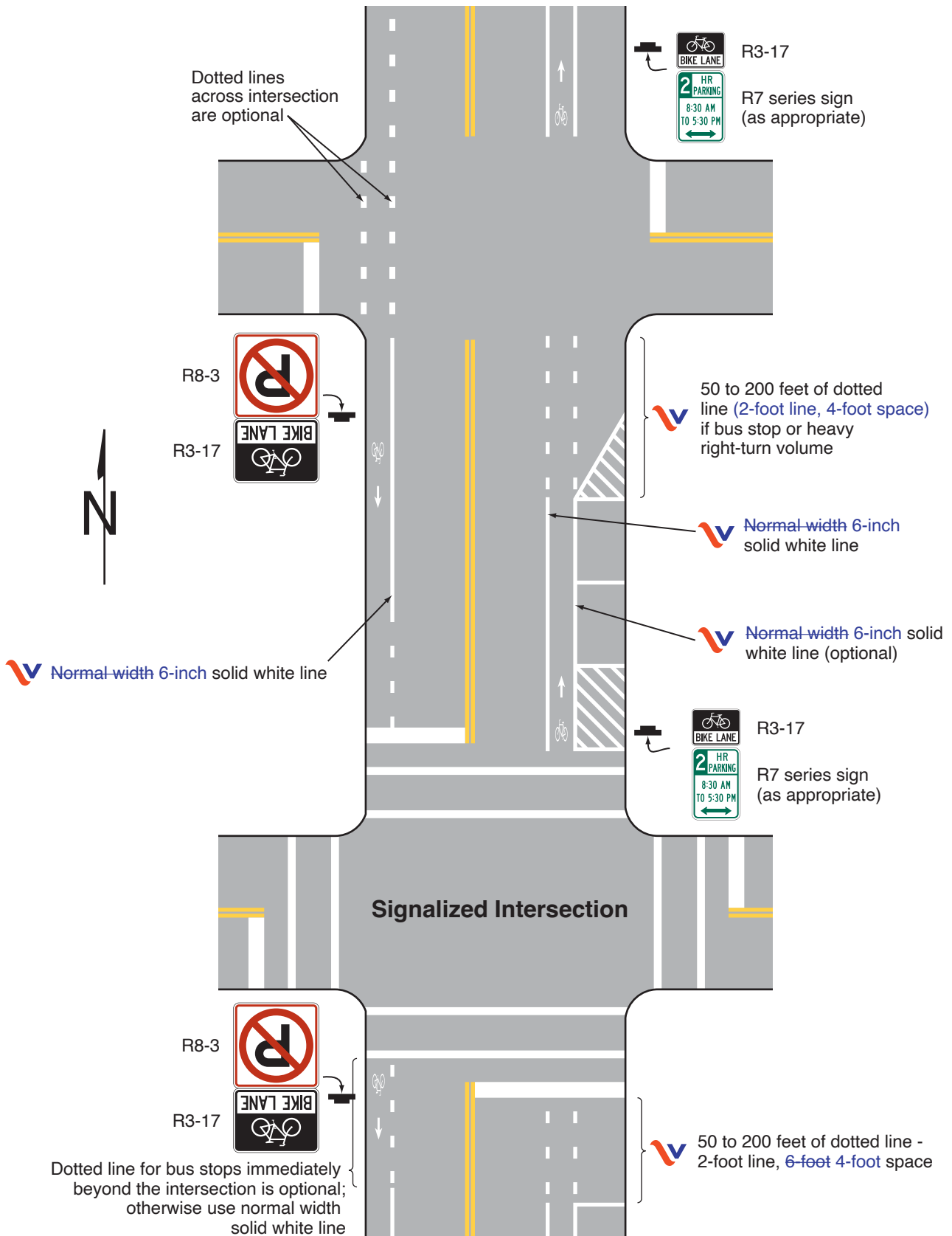
Figure 9E-2(VA). Example of Pavement Markings for Bicycle Lanes on a Two-Way Street
