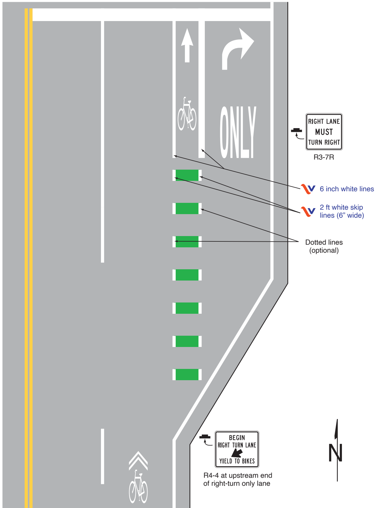
Figure 9E-4(VA). Example of Bicycle Lane Markings on an Approach to an Intersection that Transitions from a Shared Lane
